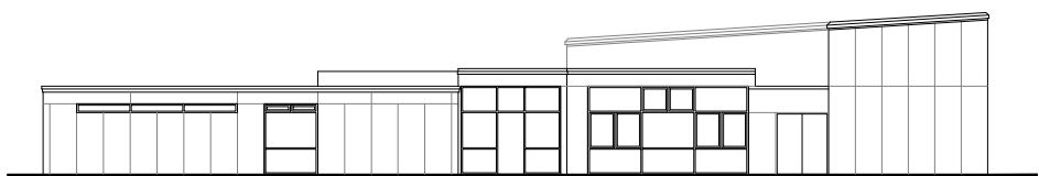
③ NORTH-WEST ELEVATION 1:100
