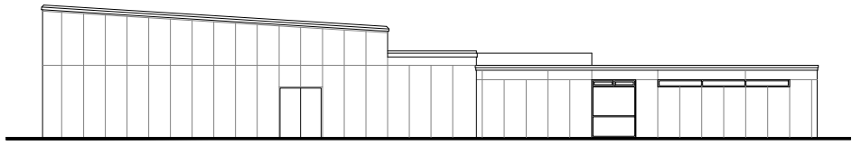
① SOUTH-EAST ELEVATION 1:100
